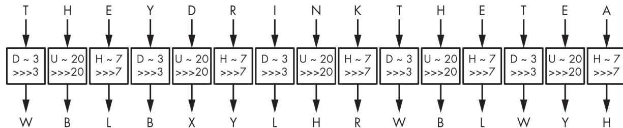
Figure 1-3: The Vigenère cipher
