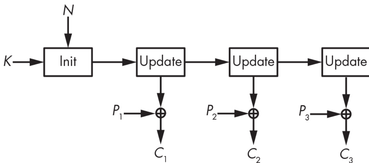
Figure 5-2: A stateful stream cipher
