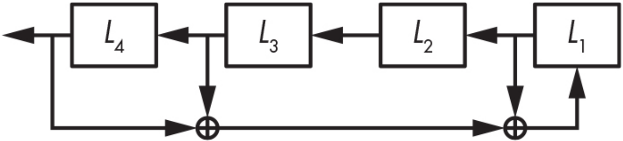
Figure 5-5: An LFSR with the feedback polynomial 1 + X + X^3 + X^4
